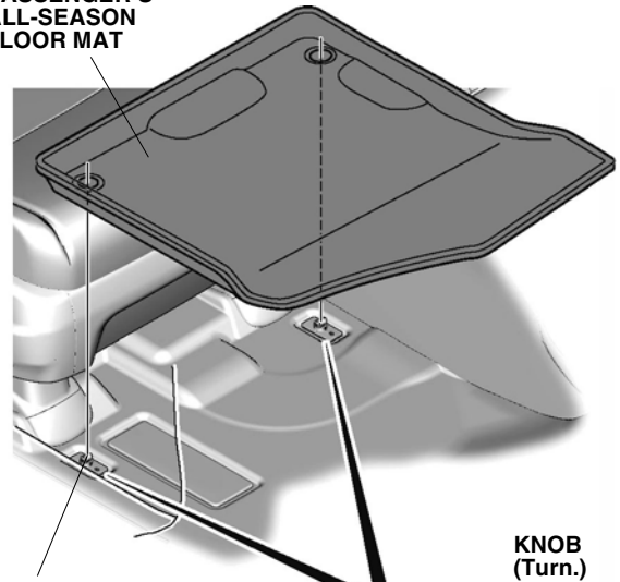
2 ANCHORS
