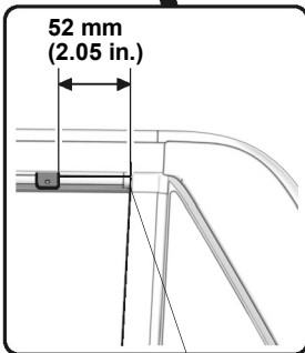
EDGE OF THE LEFT REAR DOOR REAR SASH OUTER TRIM
