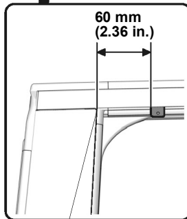
EDGE OF THE LEFT REAR DOOR SASH OUTER TRIM
