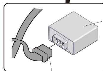
CONTROL UNIT HARNESS 12-PIN CONNECTOR
