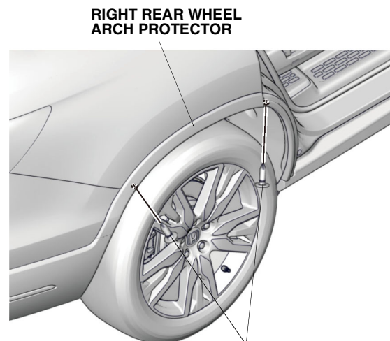
2 SELF-TAPPING SCREWS
