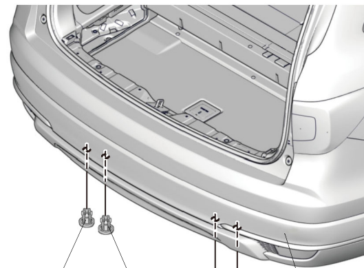
REAR BUMPER
