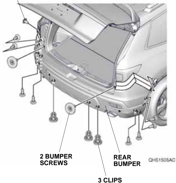
10 SELF-TAPPING SCREWS
