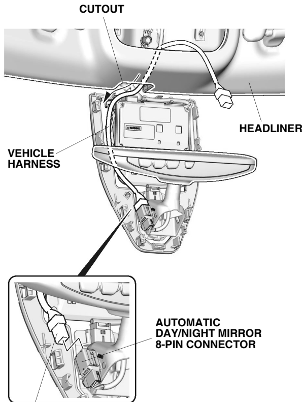
VEHICLE 8-PIN CONNECTOR
