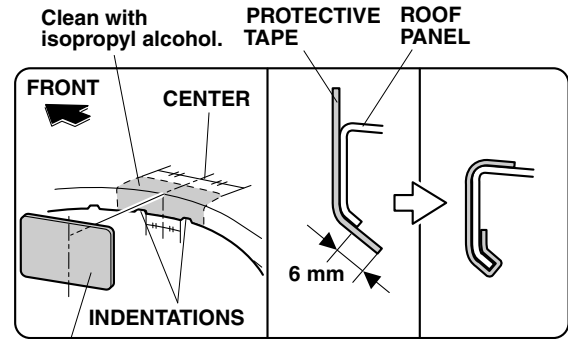
PROTECTIVE TAPE CROSS SECTION
