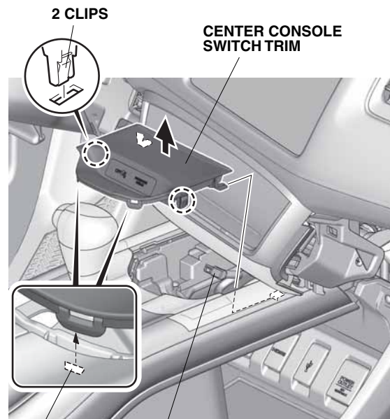
2 RETAINING TABS
