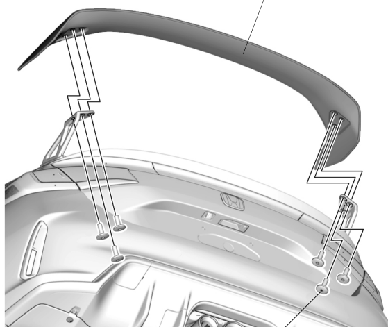
6 TORX BOLTS
