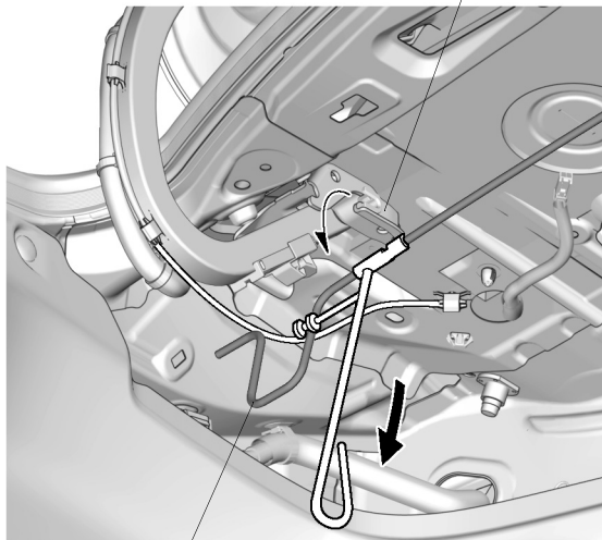
LEFT HINGE BRACKET
