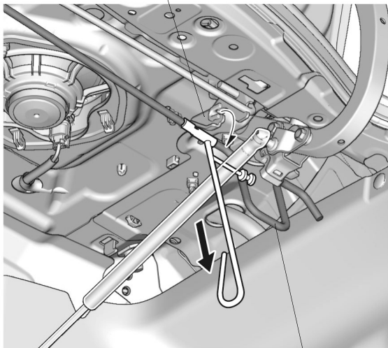
RIGHT HINGE BRACKET
