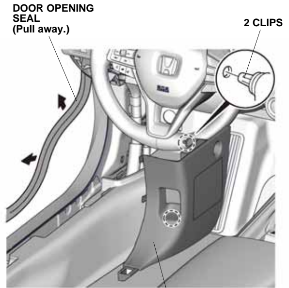
DRIVER'S KICK PANEL QG20208AG
