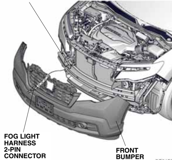
GROUND HARNESS 2-PIN CONNECTOR
