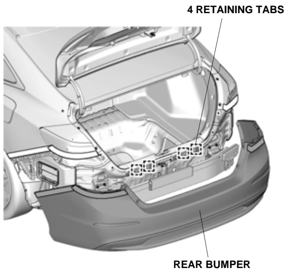
REAR BUMPER
