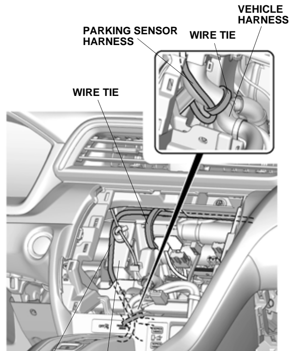
PARKING SENSOR HARNESS VEHICLE HARNESS COVER WIRE TIE VEHICLE HARNESS WIRE TIE QG01029BH
