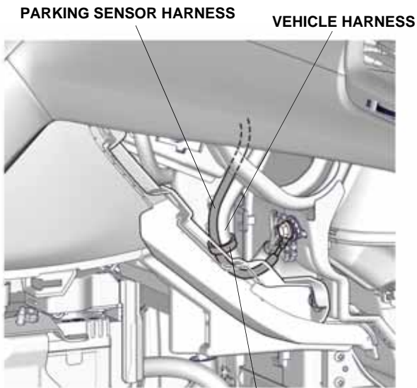
WIRE TIE PARKING SENSOR HARNESS VEHICLE HARNESS QG01027AH
