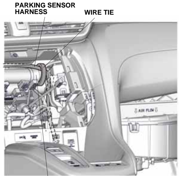
VEHICLE HARNESS PARKING SENSOR HARNESS WIRE TIE QG01028BH
