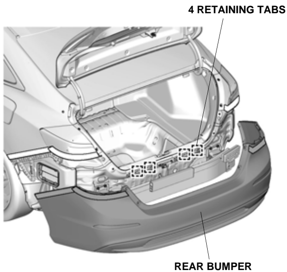
REAR BUMPER
