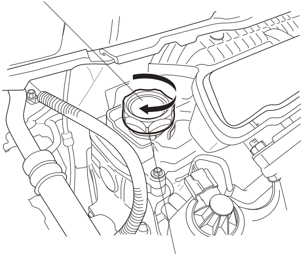
MUGEN OIL FILLER CAP (Thread until tight.)
