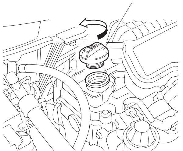
EXISTING OIL FILLER CAP (Set aside.)
