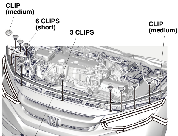
HOOD SEAL
