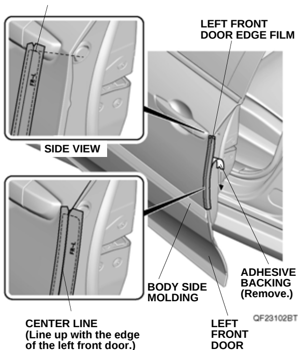
LEFT FRONT DOOR EDGE FILM (Line up with the character line.)
